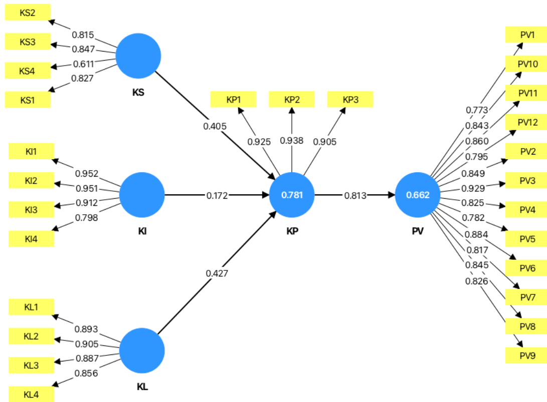
Figure 2. Structural Model (Outer Loadings, AVE, and R 2 ) - SmartPLS 4 Output
